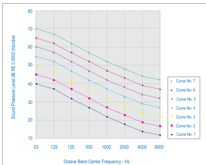
Figure 2: Approximate average minimum outdoor background sound pressure levels associated with the conditions of table D.
