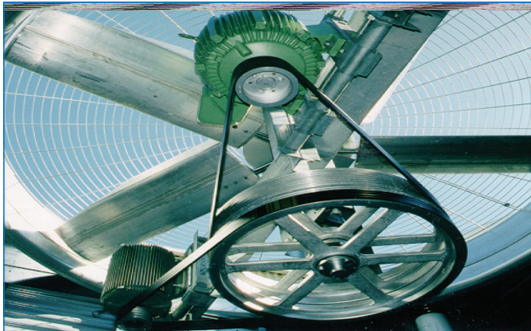
Figure 6: BAC axial fan cooling tower utilizing the Baltiguard drive
