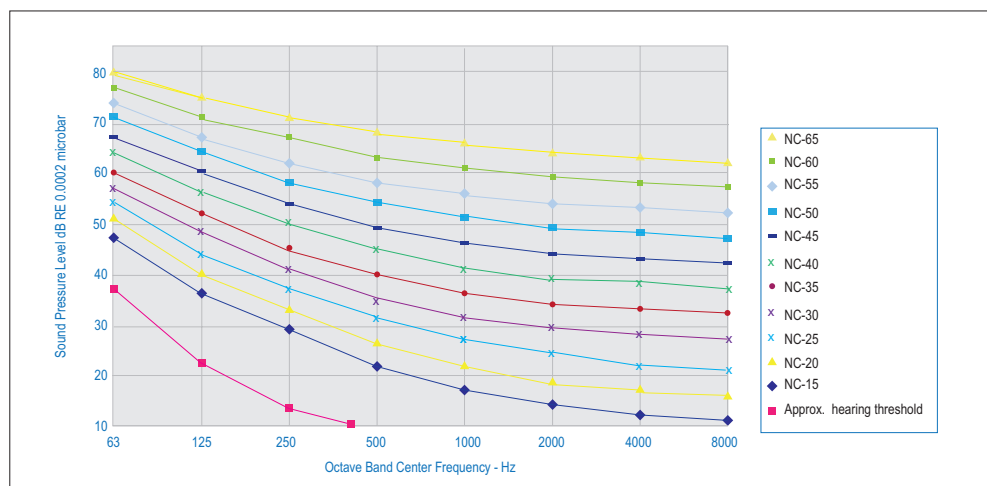
Figure 1: Noise criteria “NC” curves. The octave band sound pressure levels associated with the noise criteria conditions of Table B.
